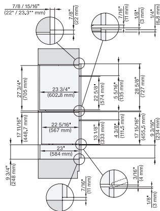
DGC7x4x+EBA7848, H7x80BP, H7x8x80BP(X), ESW7x70, EVS7670, side view, 30 Zoll, Proud, combi, XL, 650
