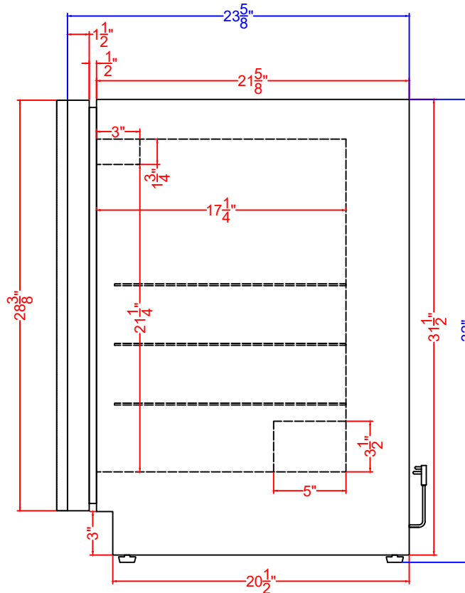
Profile View
