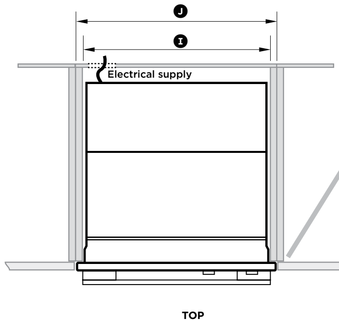
FLUSH INSTALL
