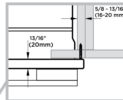
FLUSH INSTALL
