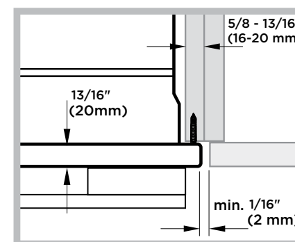
FLUSH INSTALL
