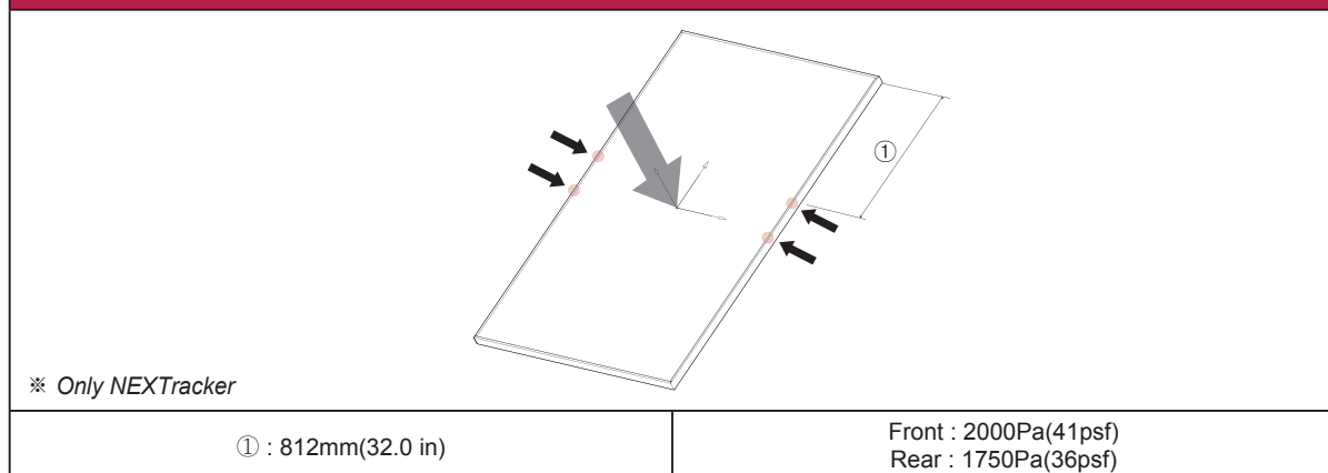
Fig7. Bolting Type
