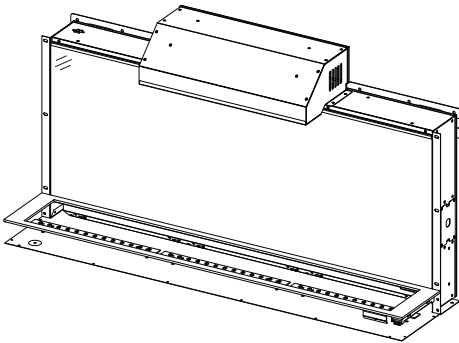
NEFLC32H E-Box
