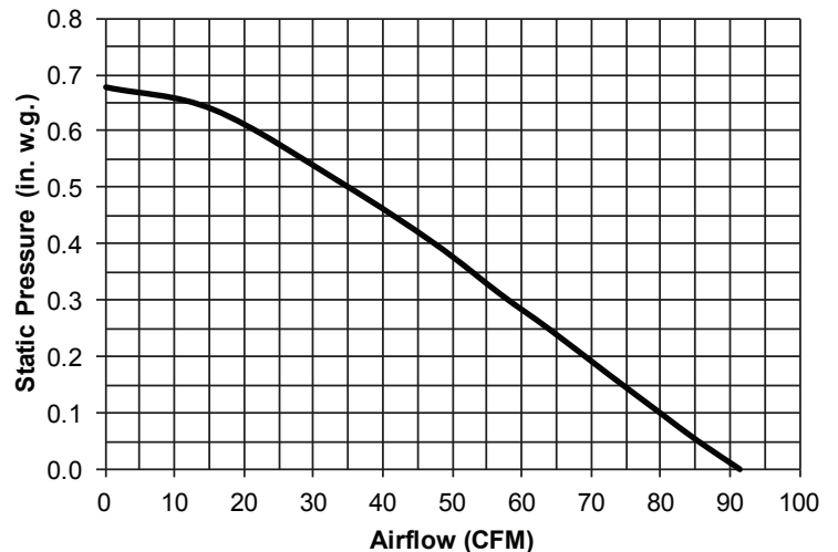
MODEL LP80 - 4" DUCT
