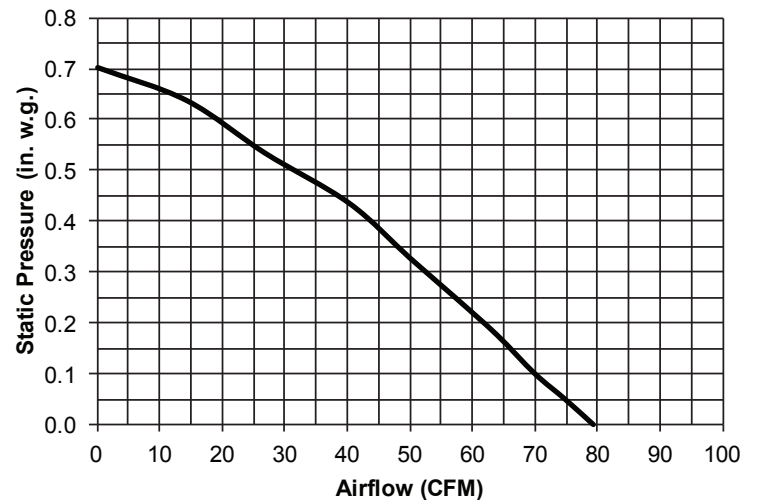
MODEL LP80 - 3" DUCT
