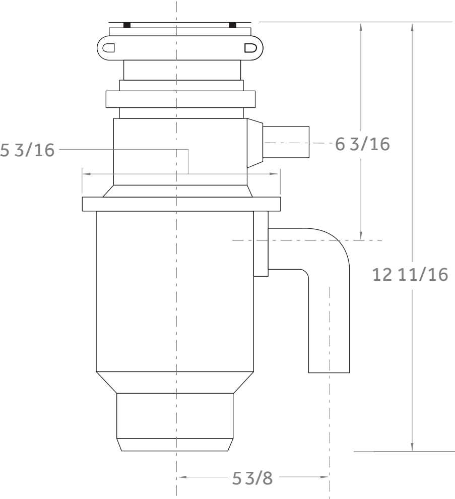
Disposall® Food Waste Disposer Dimensions (in inches)
