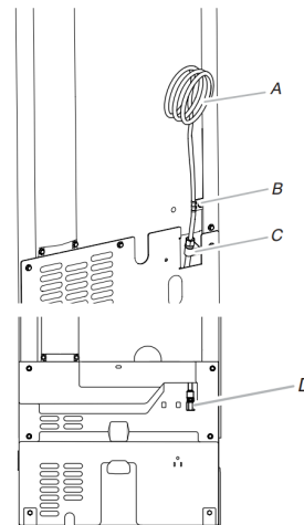
C. Inlet water tube clamp and supply line connector for standard model
