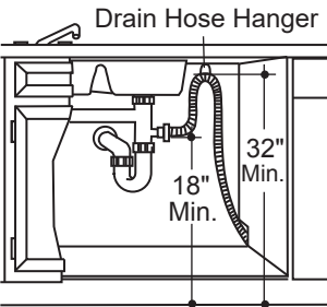
Waste Tee Installation
