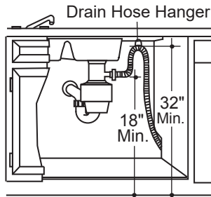
Disposer Installation
