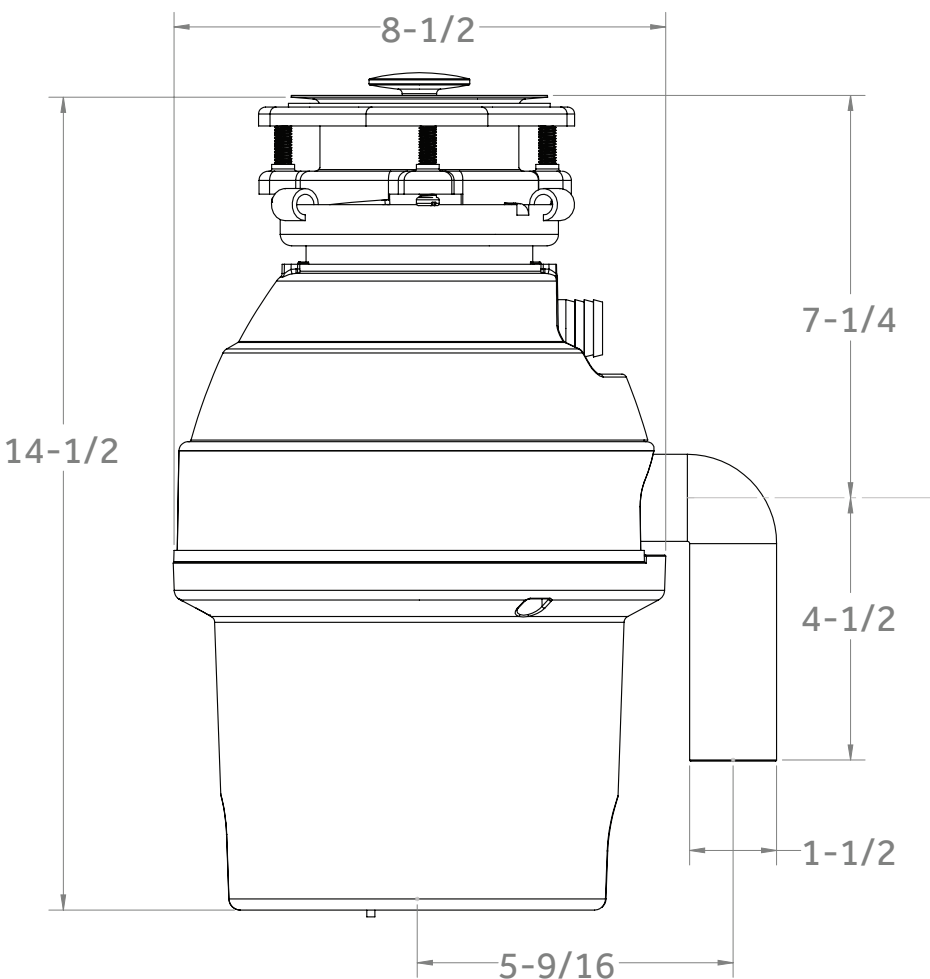
Disposall® Food Waste Disposer Dimensions (in Inches)
