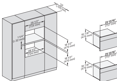
H6x80BP, H6x70BM, ESW6x85, H6x80-2BP, H7x80BP(X), H7x70BM(X), ESW7x70, EVS7670, Combi, Installation drawing, Proud, Flush inset, NA
