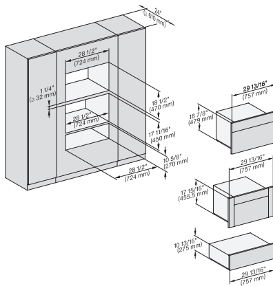
H6x70BM, H6x00BM + EBA6808, ESW6x85, DGC6x00-1 + EBA6808, NA7000 Fitting Combi wide front, Installation drawing, Proud
