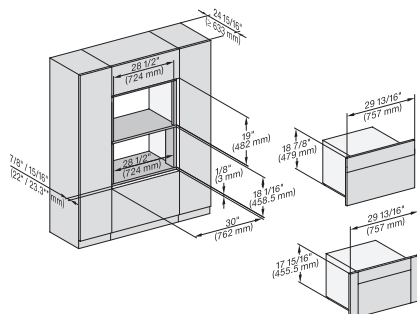
(H 6560, H 6x60) + EBA 6808; H 6x70 BM, ESW 6x85, H7xxx, EBA7868, Exx7x70, Combi, Installation drawing, Flush inset, NA
