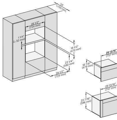
(H6560B,H6x60BP,DGC686xAM)+EBA6808,H6x70BM, DGC676x,DGC7x70,H7x6xBP+EBA7868, Fitting Combi, Installation, Proud, NA
