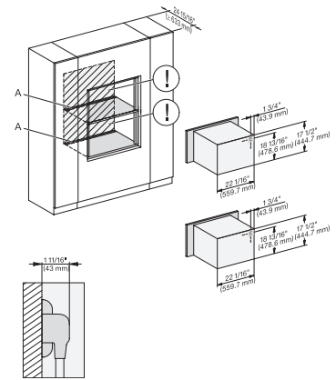
H 6x70 BM, H 7x70BM/BMX Installation Combi wide front, Installation drawing, Flush inset, NA
