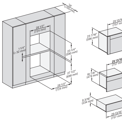
(H6560 B, H6x00 BP, H6x70 BM, DGC686x AM) + EBA6808; ESW6x85, DGC676x, NA7000, Fitting Combi w. front, drawing, Proud
