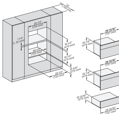
H 6x70 BM, ESW 6x85, H7x70BM(X), ESW7x80, Fitting Combi wide front, Installation drawing, Proud, NA
