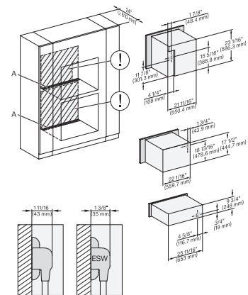
DGC786x+EBA7868, H7x70BM(X), ESW7x70, EVS7670, Installation, 30 Zoll, Flush inset, combi, wide front, XXL
