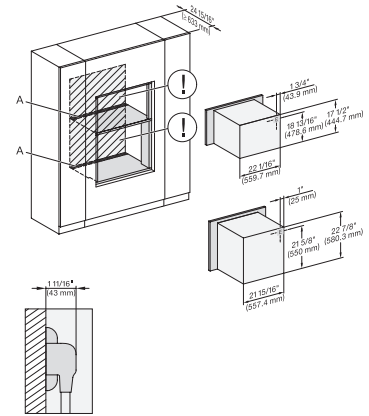
H 6560 B + EBA 6808, H 6x60 BP, H 6x70 BM, H 7xxxBM/BP/BMX, EBA 7868 Installation drawing, Flush inset, NA
