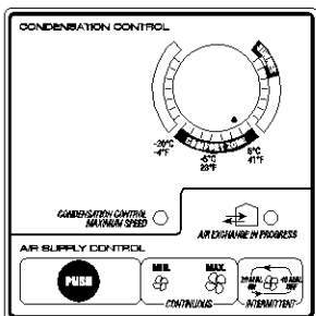
Model VT2W Electro Wall Control
