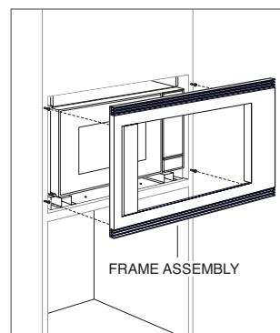
Attach assembly.
