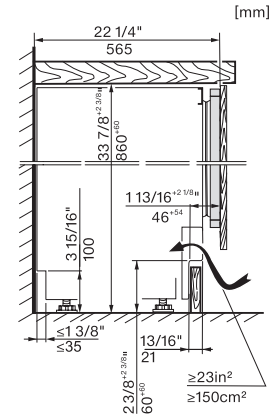
KWTUS7172F, Built-under, side view (installation drawings)
