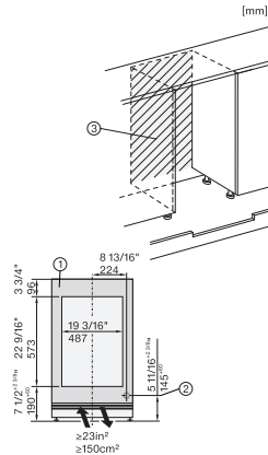
KWTUS7172F, Built-under, installation (installation drawings)
