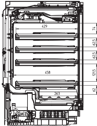
KWTUS7172F, interior dimensions (installation drawings) (US)
