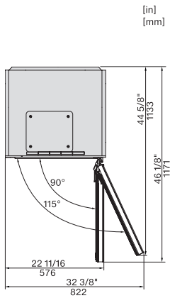
KWTUS7172F, Built-under, top view (installation drawings)
