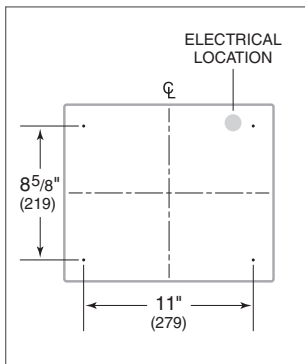
Mounting location
