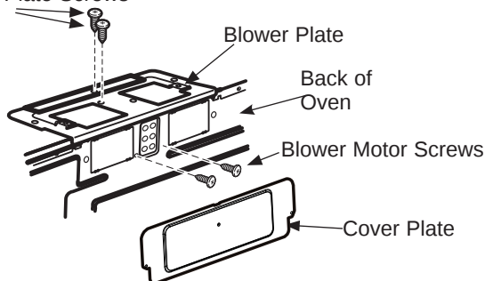
Blower Plate Screws
