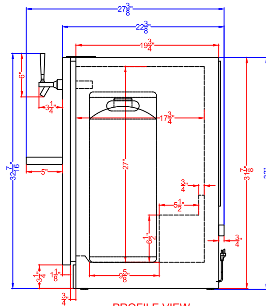
PROFILE VIEW
