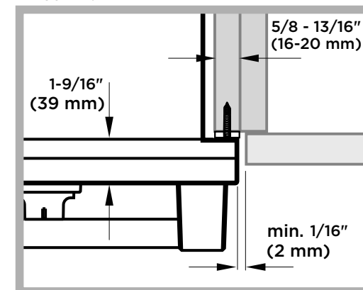
FLUSH INSTALL
