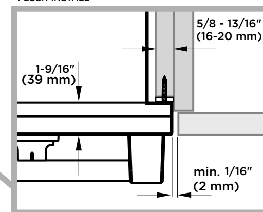
FLUSH INSTALL
