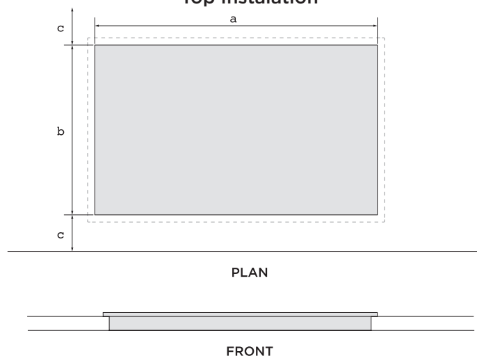
Top Installation
