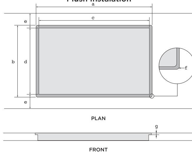
Flush Installation
