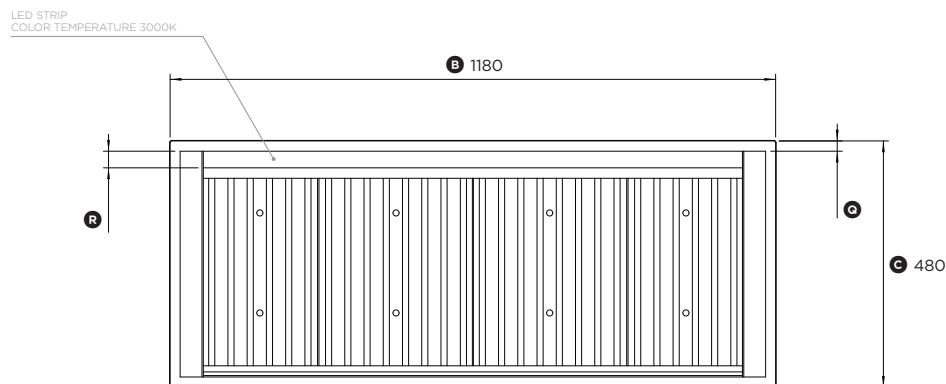
BOTTOM VIEW
