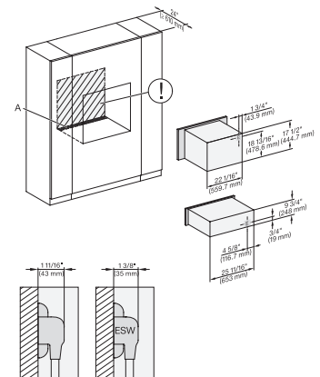
H 6x70 BM, ESW 6x85, H7x70BM(X), ESW7x70, EVS7670, Installation Combi wide front, Installation drawing, Proud, NA
