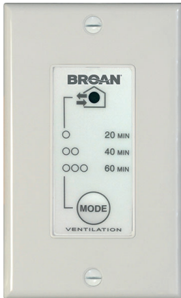
VB60W OR VBATHW PUSH BUTTON Part no. VB60W or VBATHW
