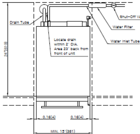
Fig. 4 Top View
