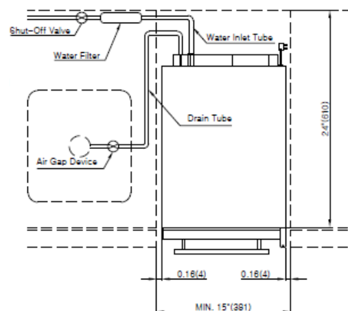
Fig. 6 Top View
