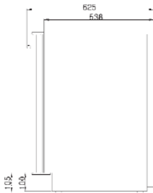
Fig. 2 Side View
