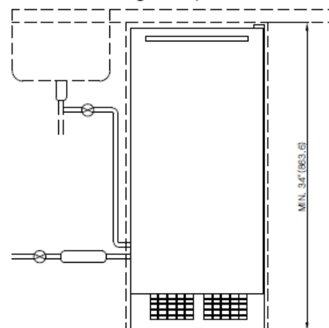
Fig. 7 Front View
