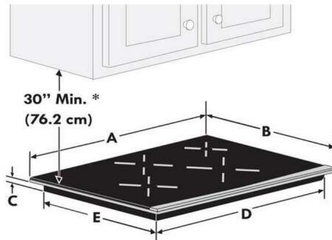
Cooktop Dimensions
