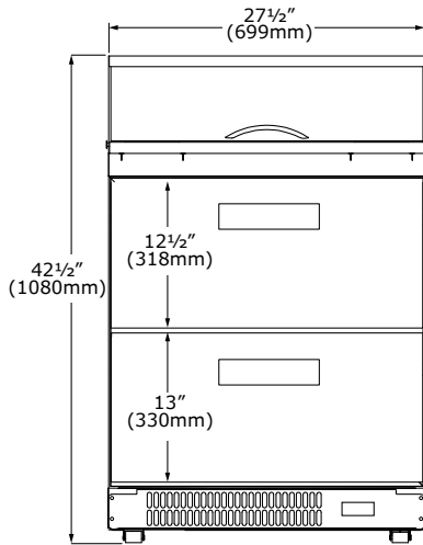
Front (UCSP127-SS91A)
