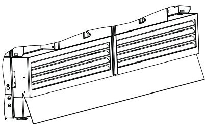
Dual Standard Custom Toe Kick Dimensions
