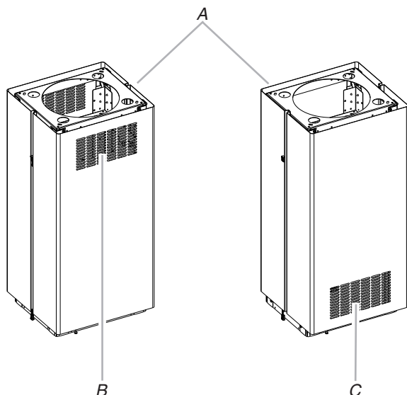
A. Top toward ceiling B. Slots installed up for non-vented installations C. Slots installed down for vented installations
