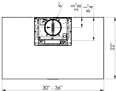
top of hood
