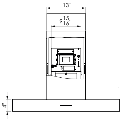
front of hood
