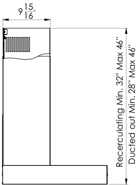
side of hood
