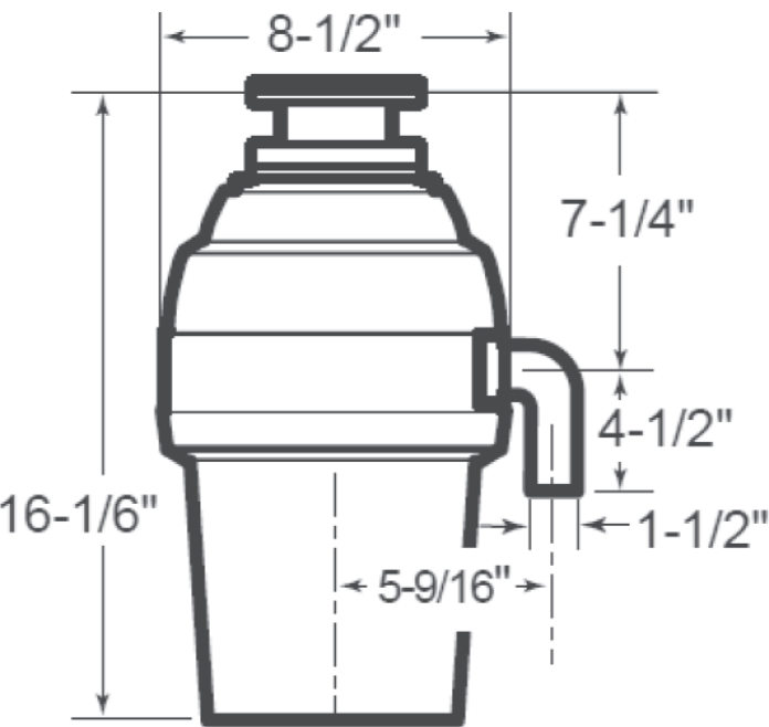
Disposall® Food Waste Disposer Dimensions (in inches)
