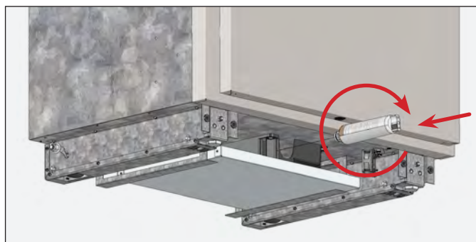
FIG. 6. Insert the water filter and rotate it clockwise.
