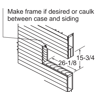
Frame Construction
