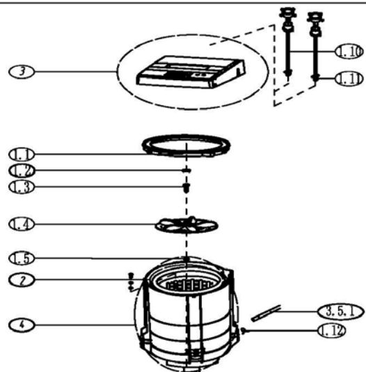
3:Top Cover Subassembly
