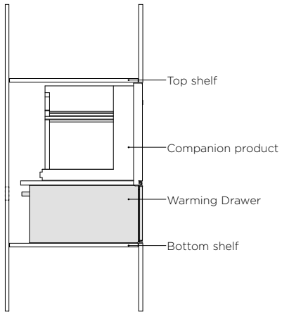
PROFILE
