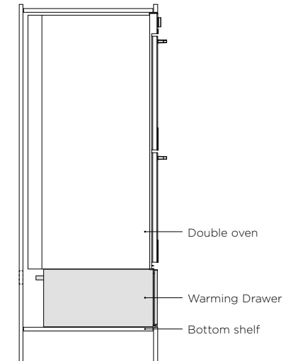
PROFILE
