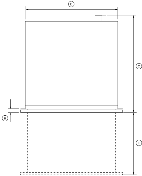
PLAN
