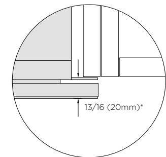
PROUD INSTALL
