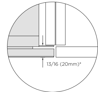
FLUSH INSTALL
