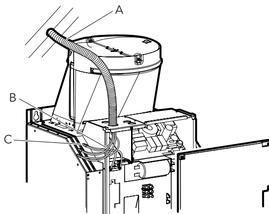
A Installation pipe B Power connection C Cable connector listed in UL
