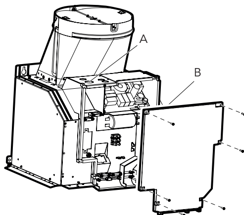
A Cable passage B Cover of the motor controller
