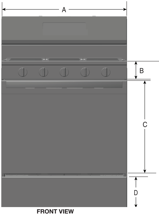
FRONT VIEW
