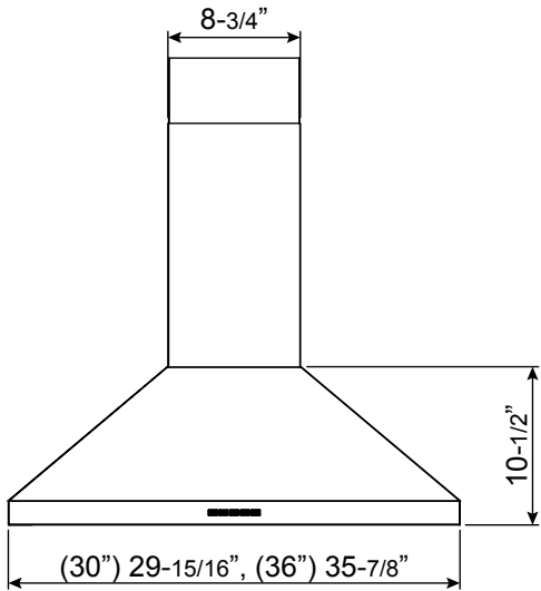
FRONT
