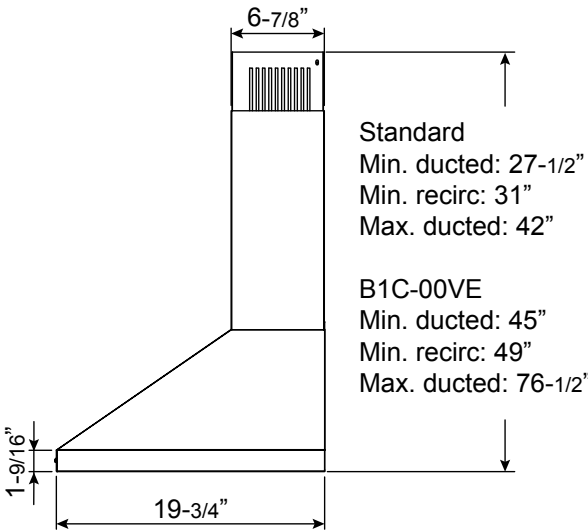
SIDE
