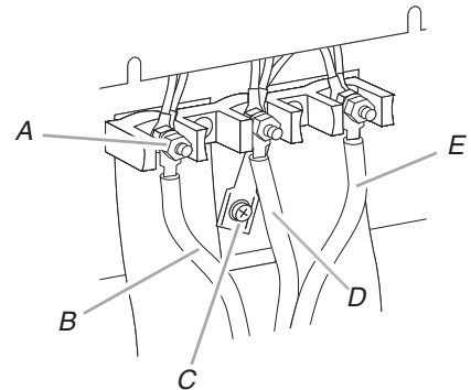
A. 10-32 hex nut B. Line 1 (black) C. Ground-link screw D. Neutral (white) wire E. Line 2 (red)
