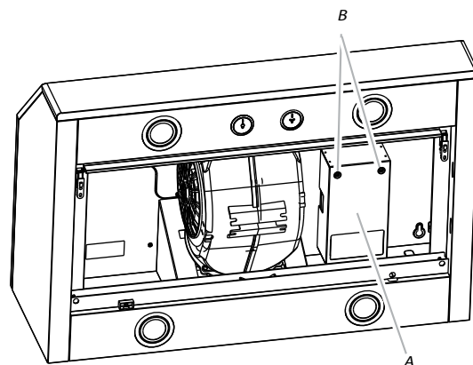
A. Terminal box cover B. Screw
