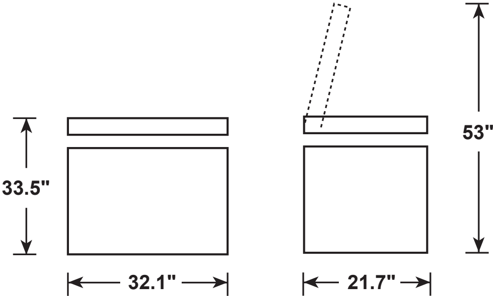
Front View
