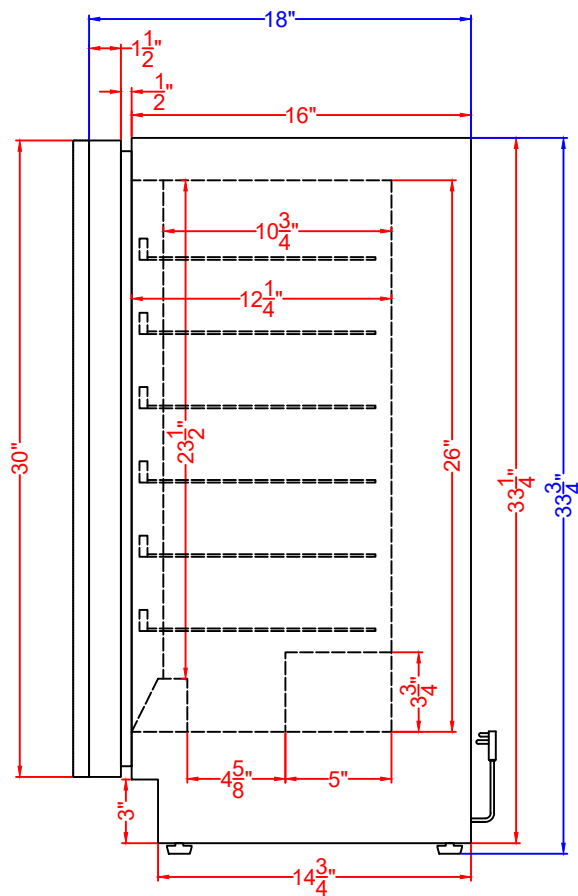
Profile View
