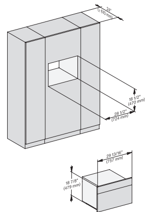
H 6x70 BM, H7x70BM(X), DG7x70(X), fitting, installation drawing, Proud, NA
