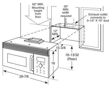
Advantium 120 above-the-cooktop oven dimensions (in inches) Models SCA1001 and SCA1000
