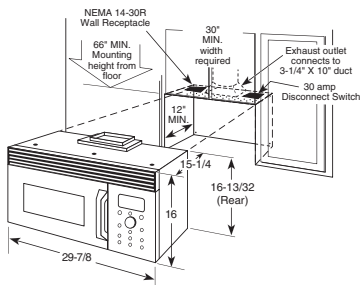
Advantium 240 above-the-cooktop oven dimensions (in inches) Models SCA2001 and SCA2000
