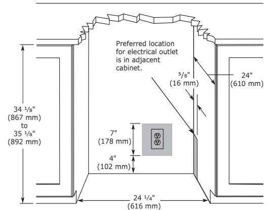
Cabinet Cut-Out
