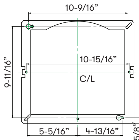
TOP SUPPORT FRAME (top view)
