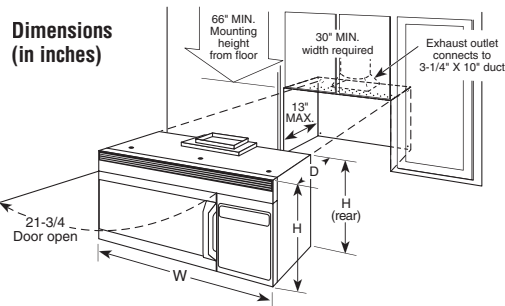
Overall Exterior Dimensions (in inches)
