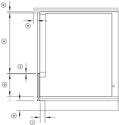
PROFILE VIEW
