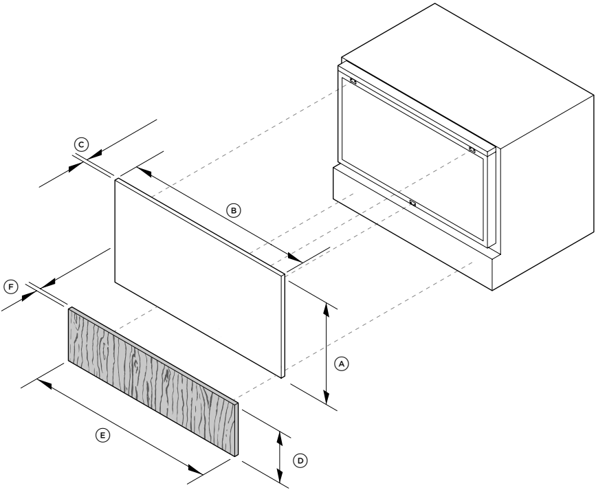
ISO VIEW
