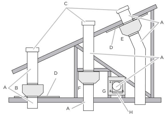
Typical In-line Blower Motor System Venting Installations
