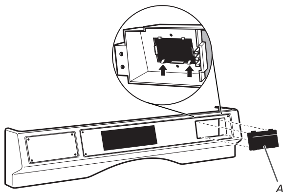
A. Card reader slot cover
