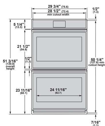
FRONT VIEW (SHOWING CUTOUT OVERLAP)
