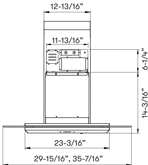
Front of Hood
