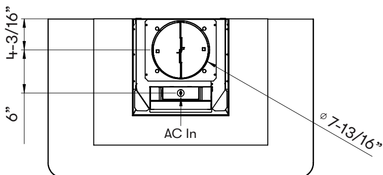
Top of Hood
