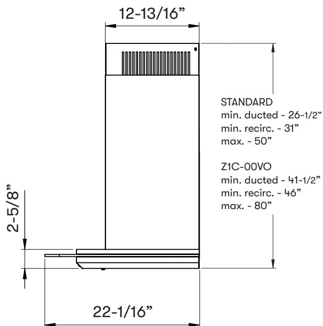
Side of Hood
